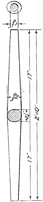
Singletree
